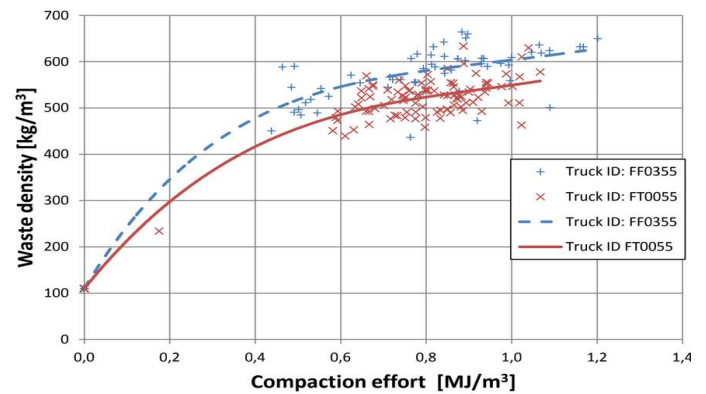
Figure 4. Compaction curves for two different compaction mechanisms
