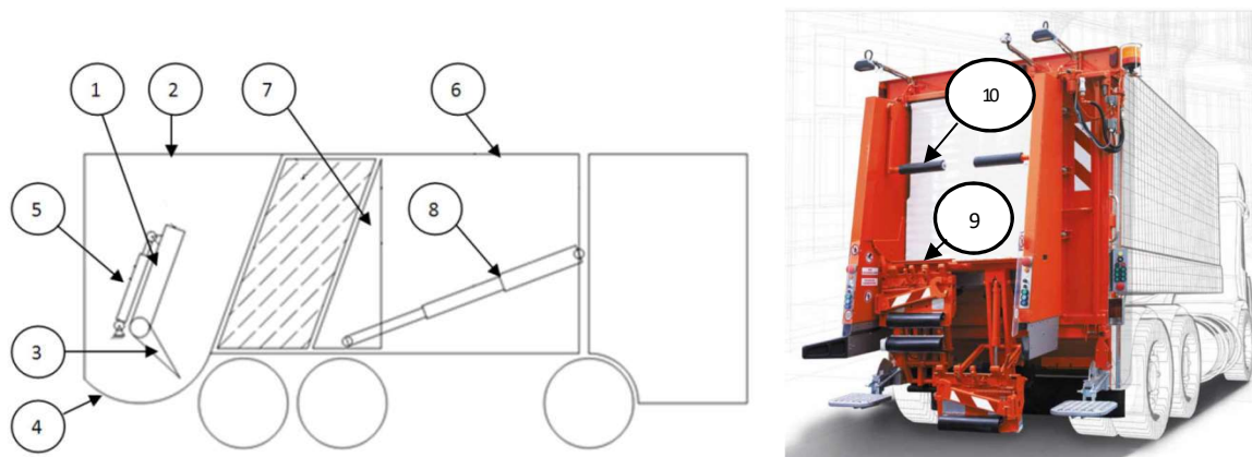
Figure 1. RCV with sweep and slide compactor; 1 - carriage plate, 2 - tailgate, 3 - packer plate, 4 - hopper, 5 - hydraulic cylinder, 6 - body, 7 - ejector plate, 8 - hydraulic telescopic cylinder, 9 - lifter, 10 - bin catcher
