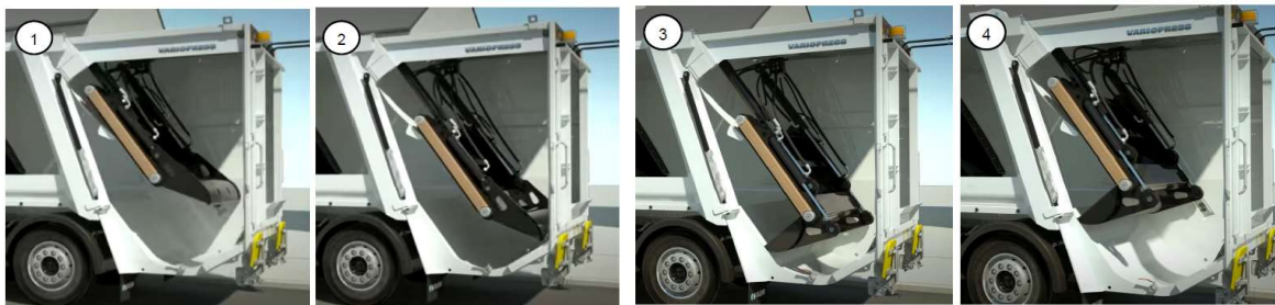
Figure 2. Operation stages of a compaction mechanism
