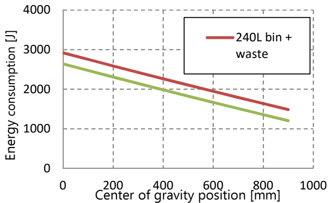
Figure 9. Relationship between energy consumption and height of the centre of gravity of waste
